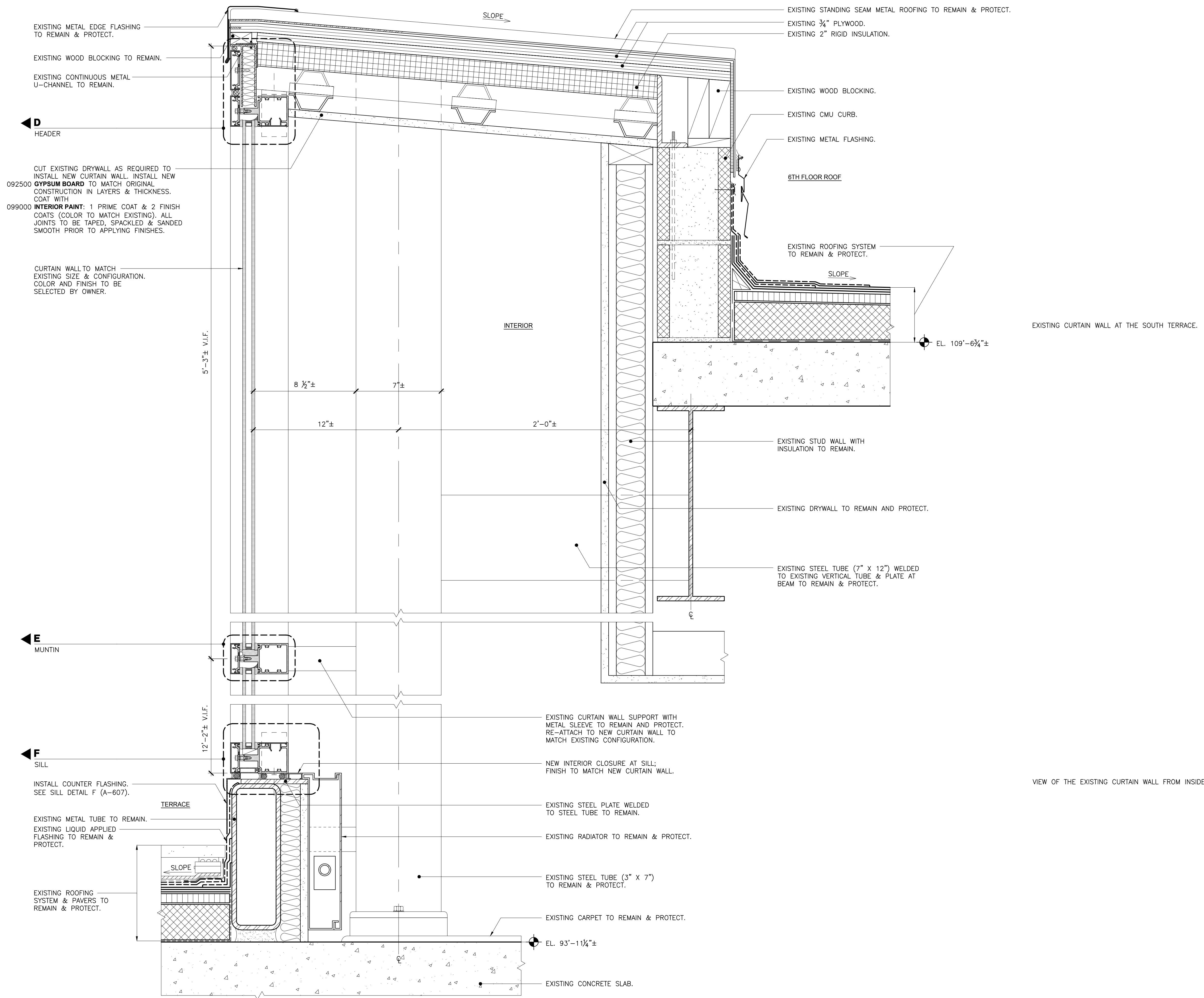
SECTION B-B
